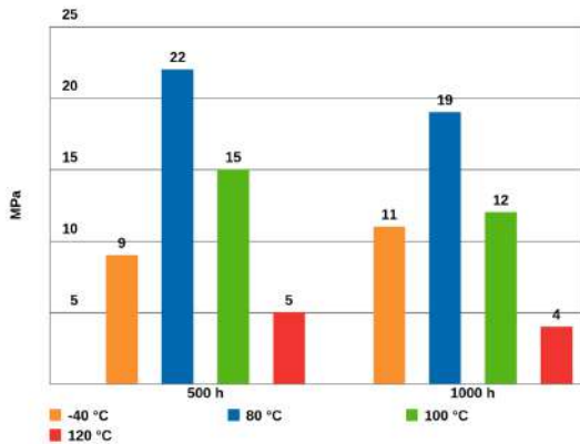
Compression shear strength after temperature storage Substrates: glass/ glass, by the criteria of DELO Standard 5
